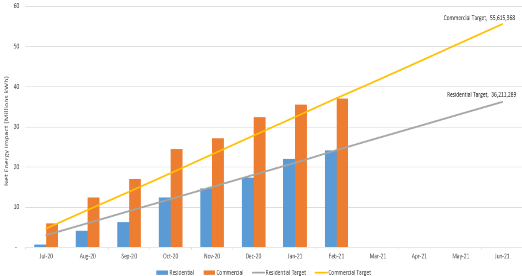
Chart 3: PY2020 Net Energy Impact Tracking (First Year)
